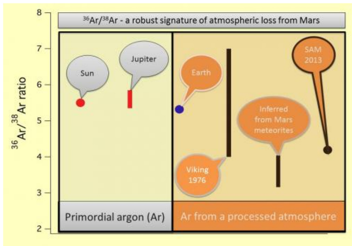
This image shows the ratio of the argon isotope argon-36 to the heavier argon isotope argon-38, in various measurements. Image: NASA/JPL-Caltech
