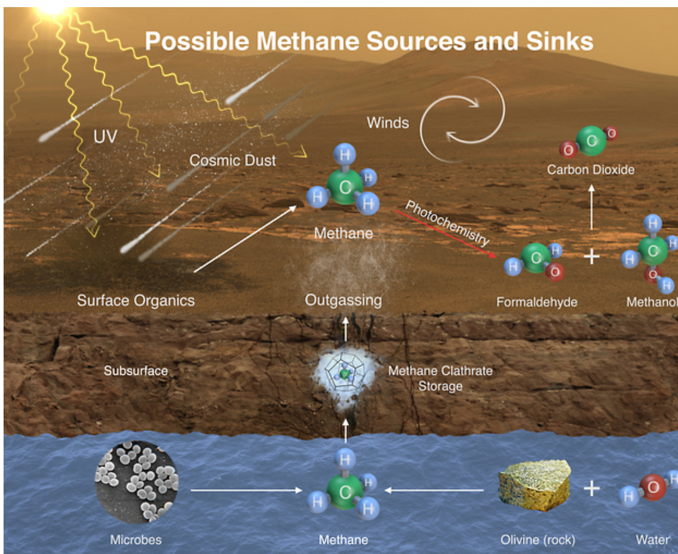
This image illustrates possible ways methane might be added to Mars' atmosphere (sources) and removed from the atmosphere (sinks). NASA's Curiosity Mars rover has detected fluctuations in methane
